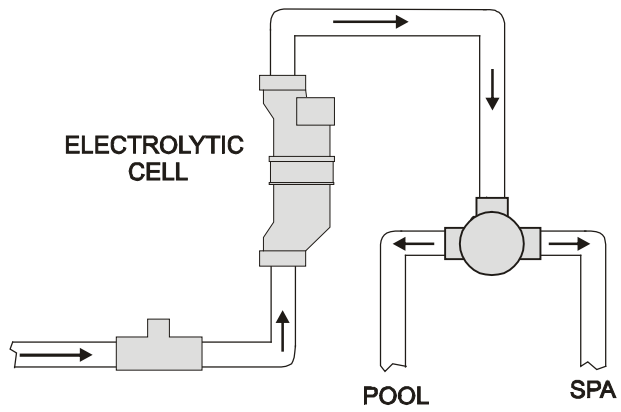
Vertical Installation
