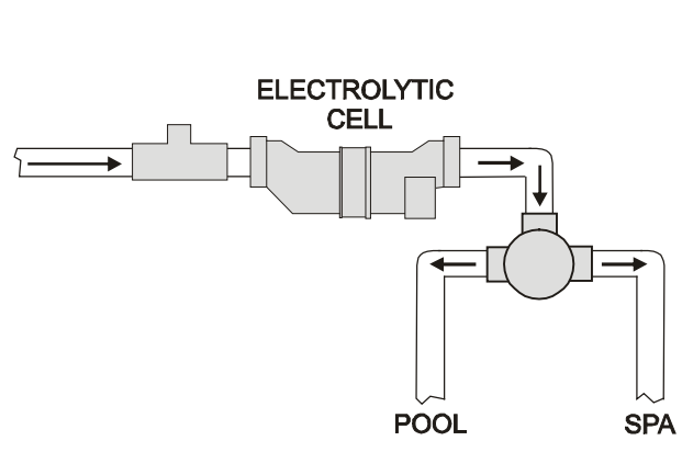
Inverted Installation
