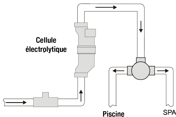
Installation verticale
