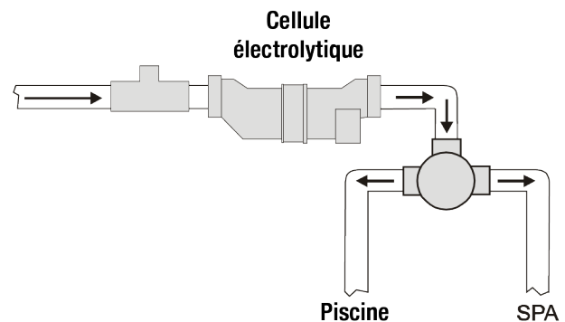
Installation inversée
